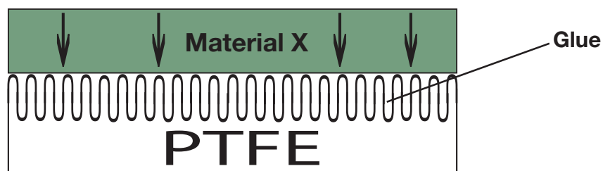
fig. 69: gluing PTFE
