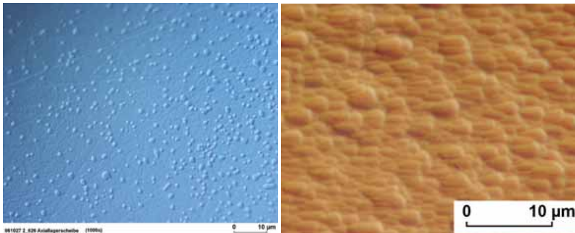
fig. 81: DLC layer with nano scale insitu structure
