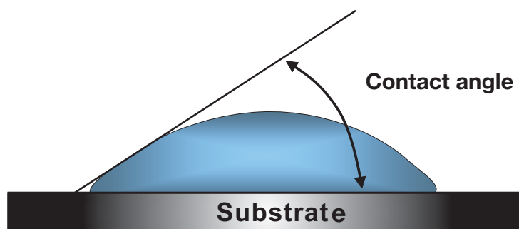
fig. 36: contact angle
