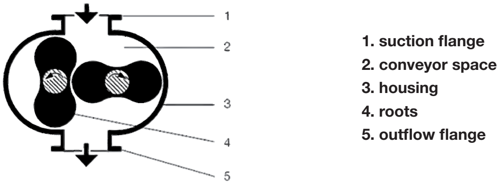
fig. 122: schematic cut of a roots pump
