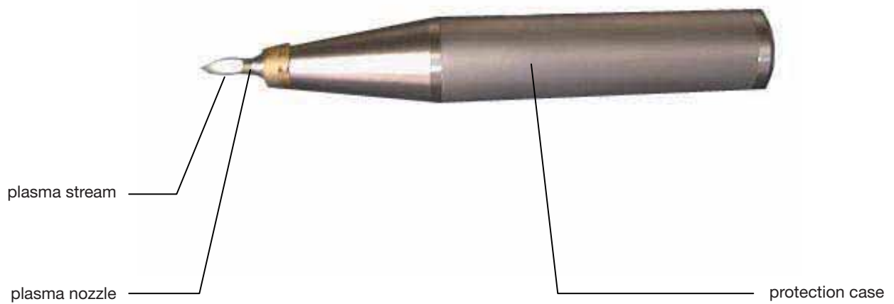
fig. 172: plasma device
