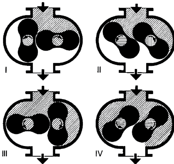
fig. 123: method of function of a roots pump
