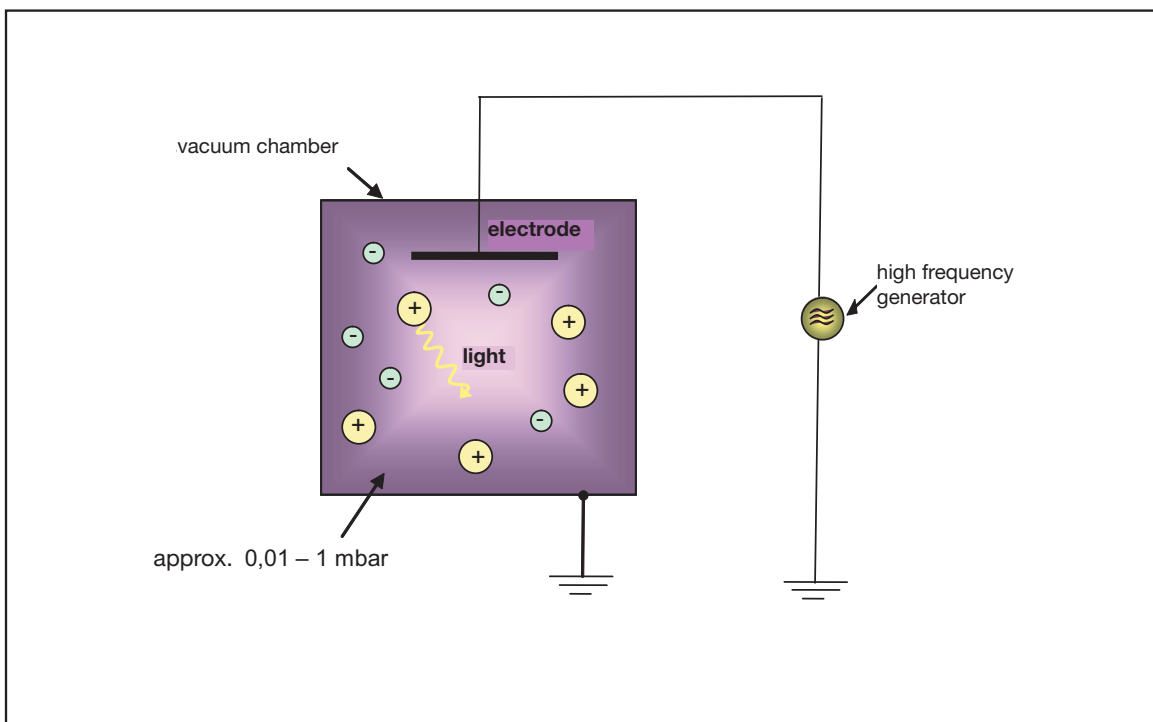
fig. 15: schematics of a plasma chamber
