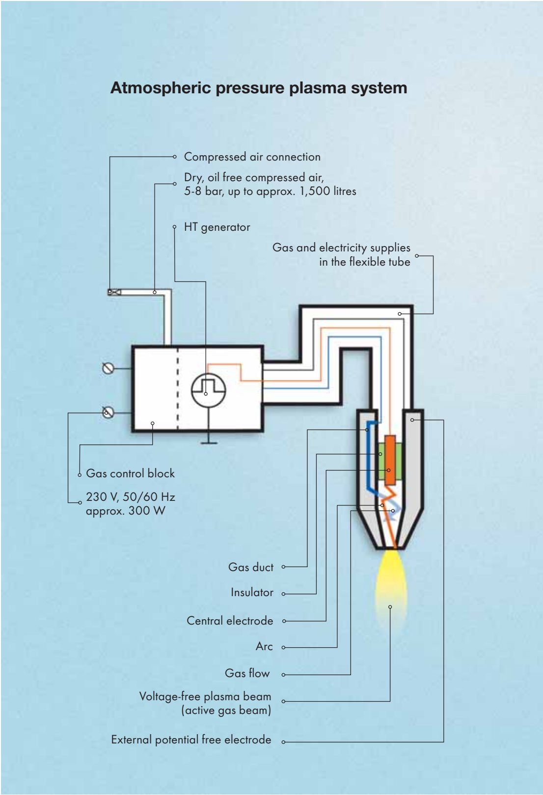
fig. 168: functional principle of a atmospheric plasma system
