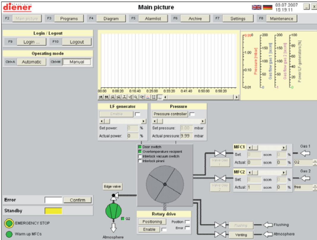
fig. 114: manual operation
