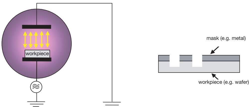
fig. 150: RIE operation
